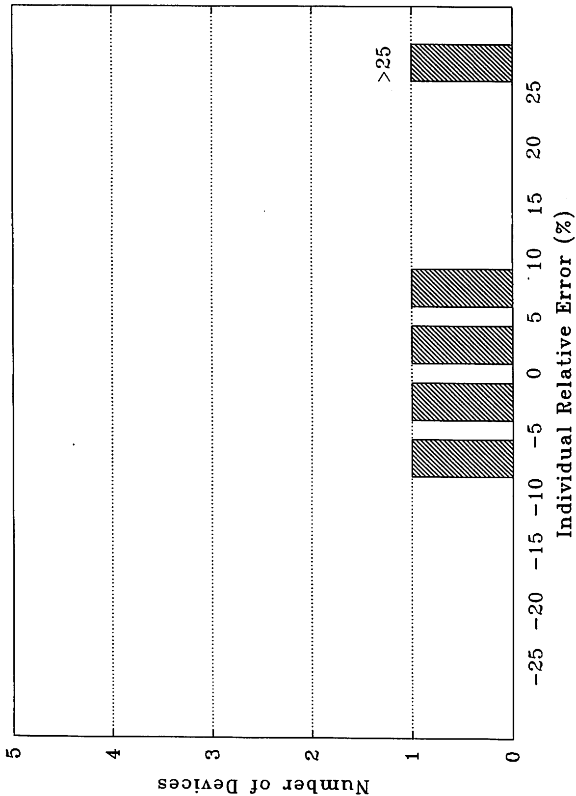
Fig. 5. Distribution of Relative Errors for Radon Progeny Monitors
