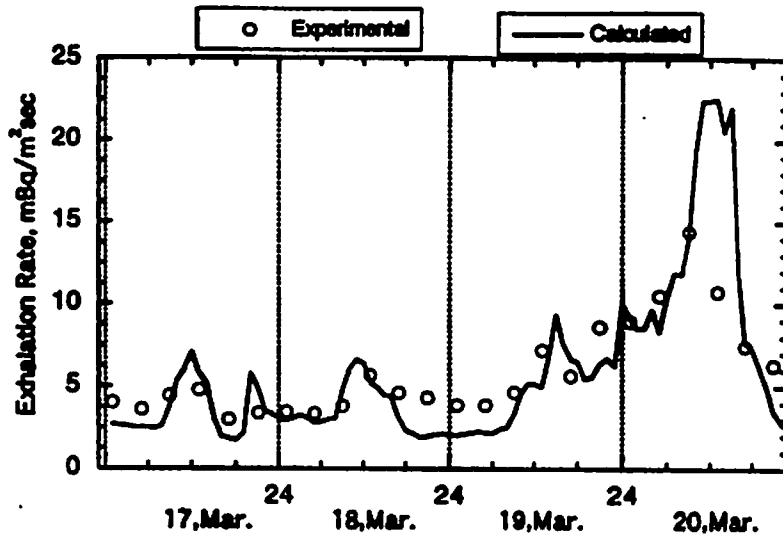
Fig.7(a). Time variation of experimental and simulated radon exhalation rates.
