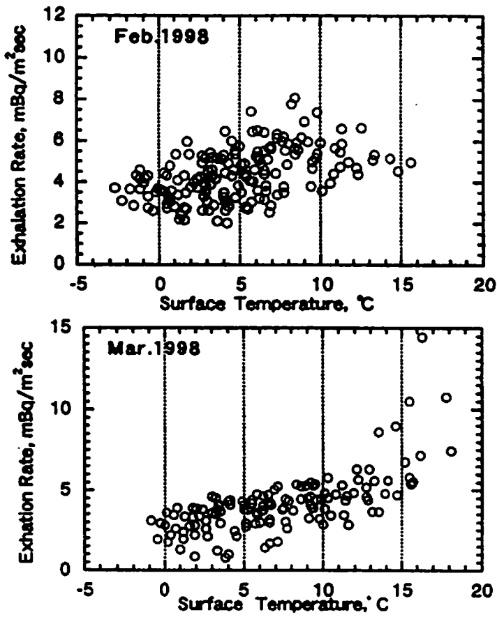
Fig.5. Scatter plots of exhalation and surface temperature.
