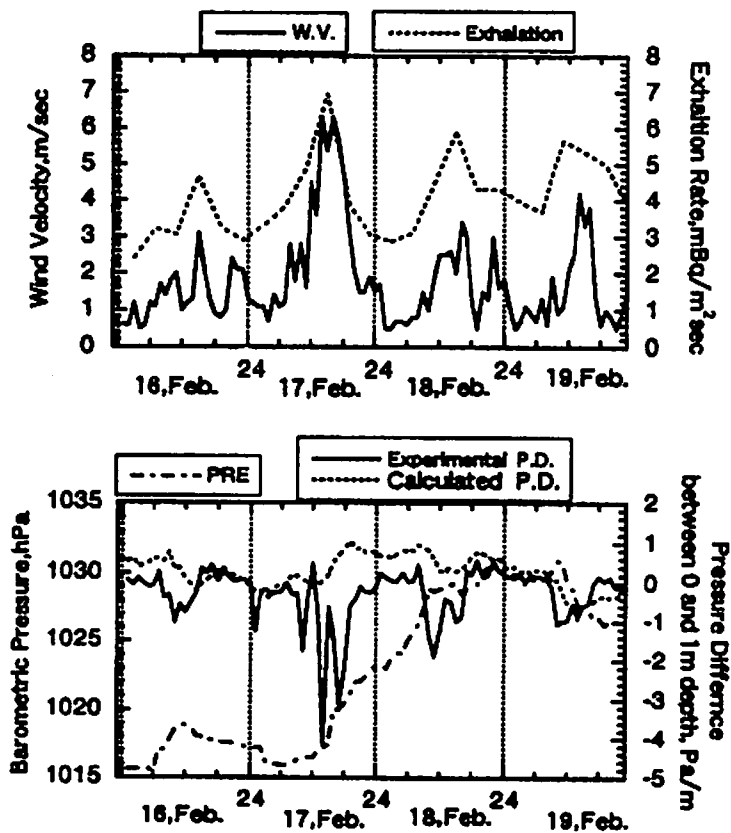
Fig.4. Time dependent measurements for exhalation, wind velocity(W.V.), barometric pressure(PRE) and pressure difference(P.D.) between surface and 1 m depth.
