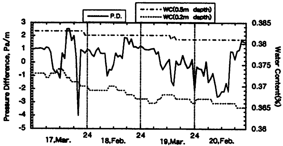
Fig.7(b). Time variations of hourly data of pressure difference and water content at 0.2 and 0.5 m depths, used for this simulation.
