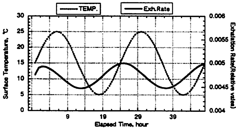
Fig.6. calculated radon exhalation rate when the surface temperature has sinusoidal variation.
