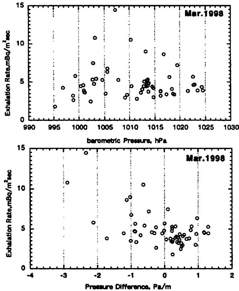
Fig.2. Relation between exhalation rates and barometric pressure (above) and pressure difference(below), during Mar.1998
