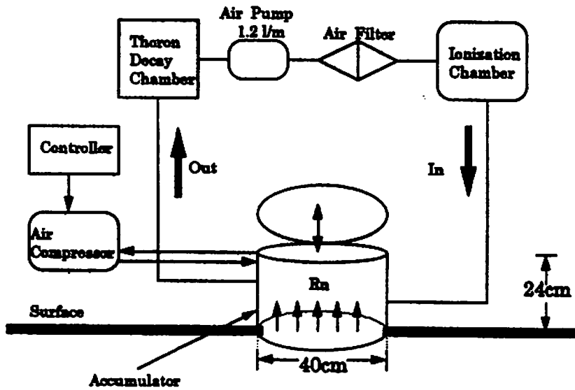
Fig.1. Experimental arrangement of radon exhalation.
