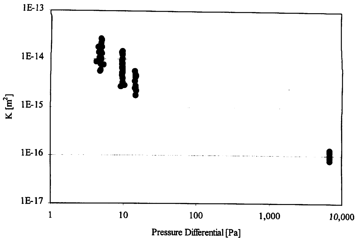
Fig. 4. Experimental results of air permeability coefficient versus applied pressure difference.
