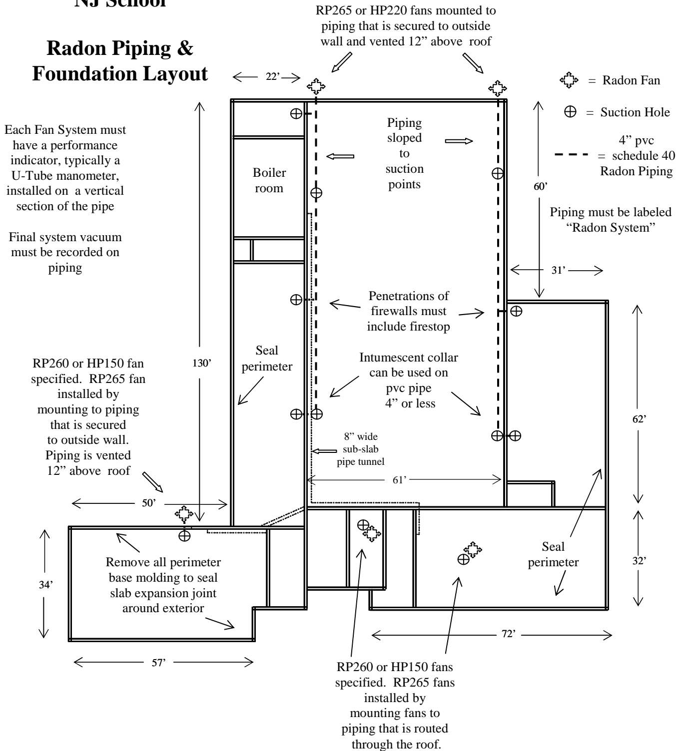
Figure 2. Foundation plan showing sub-slab divisions and final radon re-remediation piping and fan locations. Total interior perimeter and visible expansion joints sealed.
