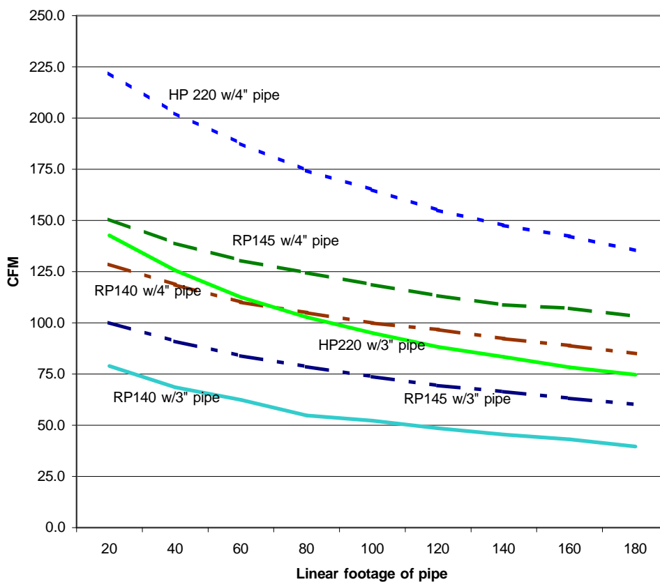
Maximum Fan CFM capacity with different open Pipe
