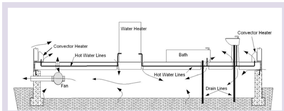
Figure 14 – Crawlspace Exhaust
