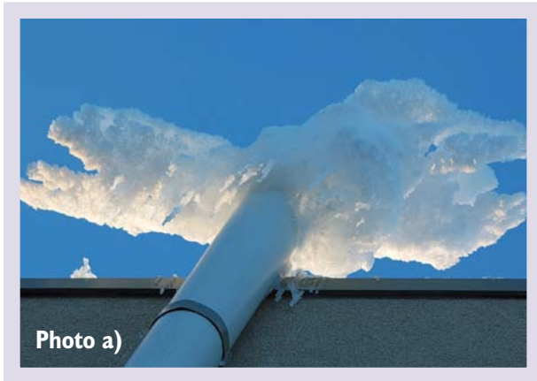
Examples of sub-slab depressurization system with a roof exhaust stack a) Ice build-up on a un-insulated system b) Insulated system with fan in the attic
