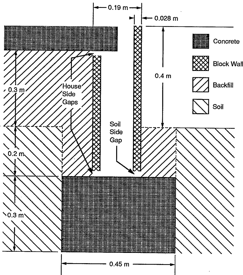
Figure 2. Detail of the stem wall, showing the fixed dimensions for the wall height, dimensions of the footing, and fill depth and location. The size of the gaps at the top and bottom of the stem wall is exaggerated in this diagram. In the base case, their widths are 3 mm. The floor slab thickness is 10 cm.
