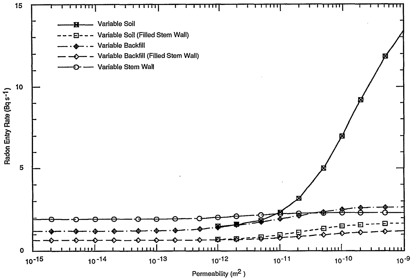
Figure 3. Range of radon entry rates produced by variations in the soil, fill, and stem wall permeabilities for open and concrete-filled stem walls. Also shown are entry rates when the stem wall/footing gap is eliminated. In each case, all other parameters have the base case value.
