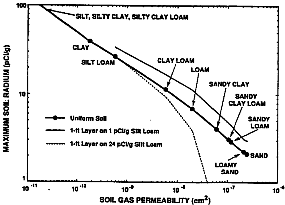
Figure 3. Maximum soil radium concentrations to maintain 2 pCi/liter radon in a slab-on-grade structure (Figure 1) on SCS soils that are uniform (solid line) or used for 1 ft fill layer over a silt-loam base soil (broken lines).
