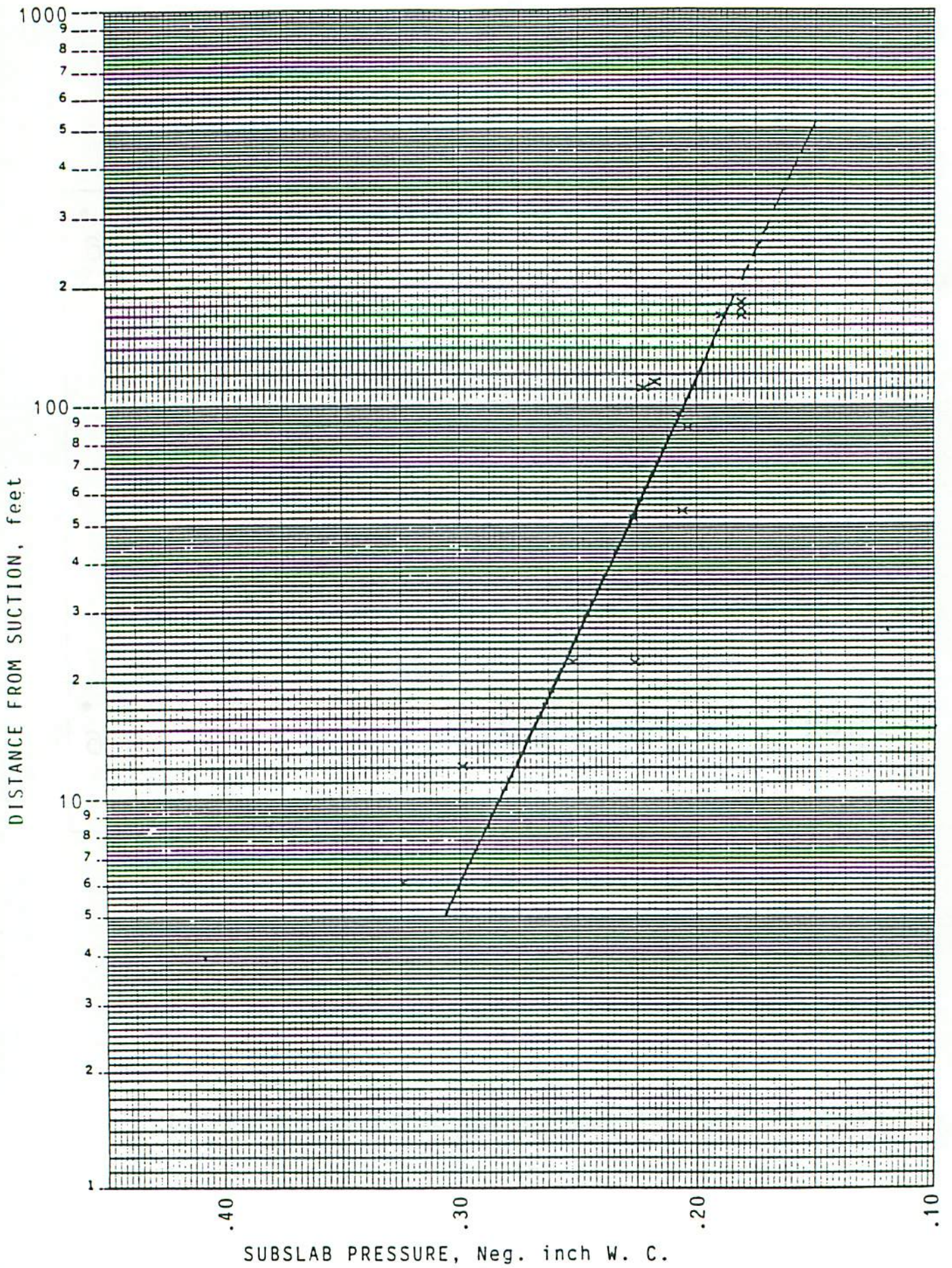
Figure 10. Pressure field extension for complete slab
