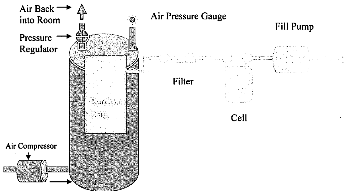
Figure 5: An air compressor brings the chamber to a desired pressure. The pressure is maintained to within 0.01 pound per square inch with a gauge and a regulator. Using a second, independent pump, the radon is extracted from the bag (under pressure), filtered and flowed through the Rocky Mountain cell.
