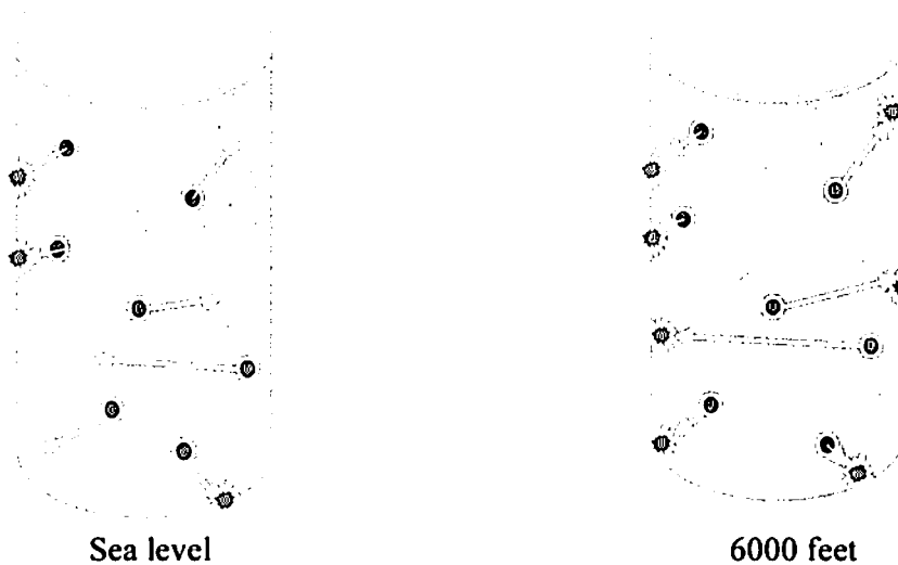
Figure 1: On the left, of the seven alpha particles being made during a one-second interval, only three can travel far enough to strike the sensitive surface of the interior of the cell. At 6000 feet, the cell on the right is filled with the same concentration of radon and radon decay products and the seven alpha particles being made during an equivalent one second interval all strike the sensitive surface of the interior of the cell and are counted.
