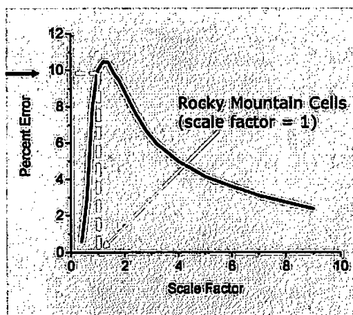
Figure 3: A theoretical model which predicts the error resulting from using a given cell at sea level and again at 6000 feet. The largest theoretical error occurs for the Rocky Mountain cell, the most common cell used in the radon industry and the standard cell used in intercomparisons.
