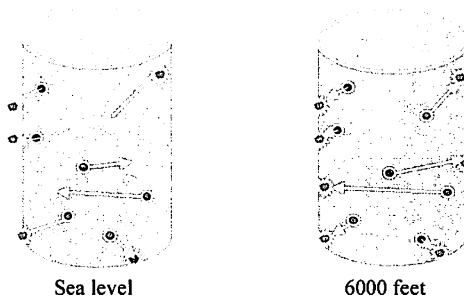
Figure 2: For the same radon concentration, the cell on the left, still at sea level, now has five alpha particles striking the zinc sulfide surface. The only difference between this example and the example in figure 1 is that both cells are now smaller. This allows more alpha particles to strike the left hand cell at any air density (elevation).
