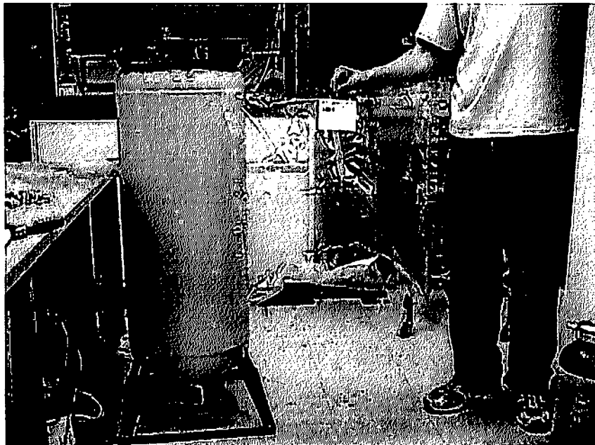
Figure 4: The pressure chamber and the large flexible bag. The bag will be filled with radon and inserted into the chamber, which is then sealed.
